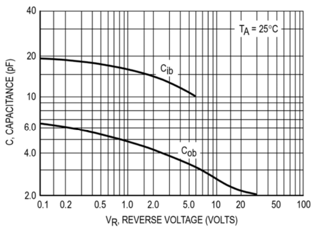
Capacitance
